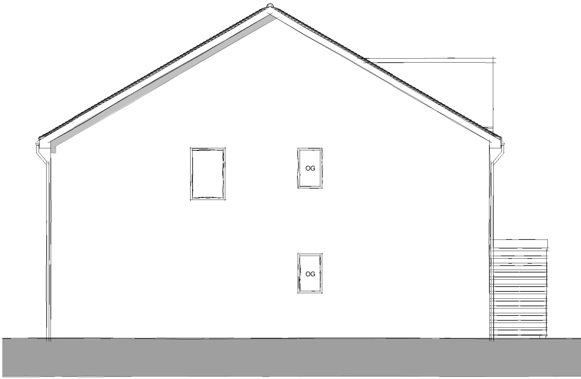
LHS Elevation 1:100
